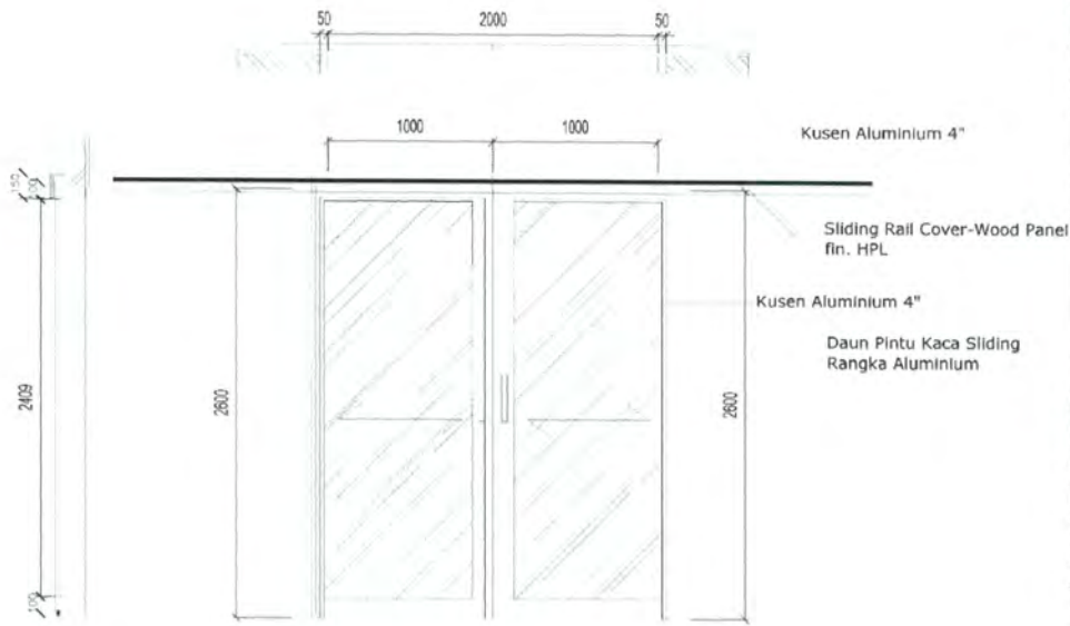
DETAIL PINTU SLIDING (PS2) Scale: 1/20
